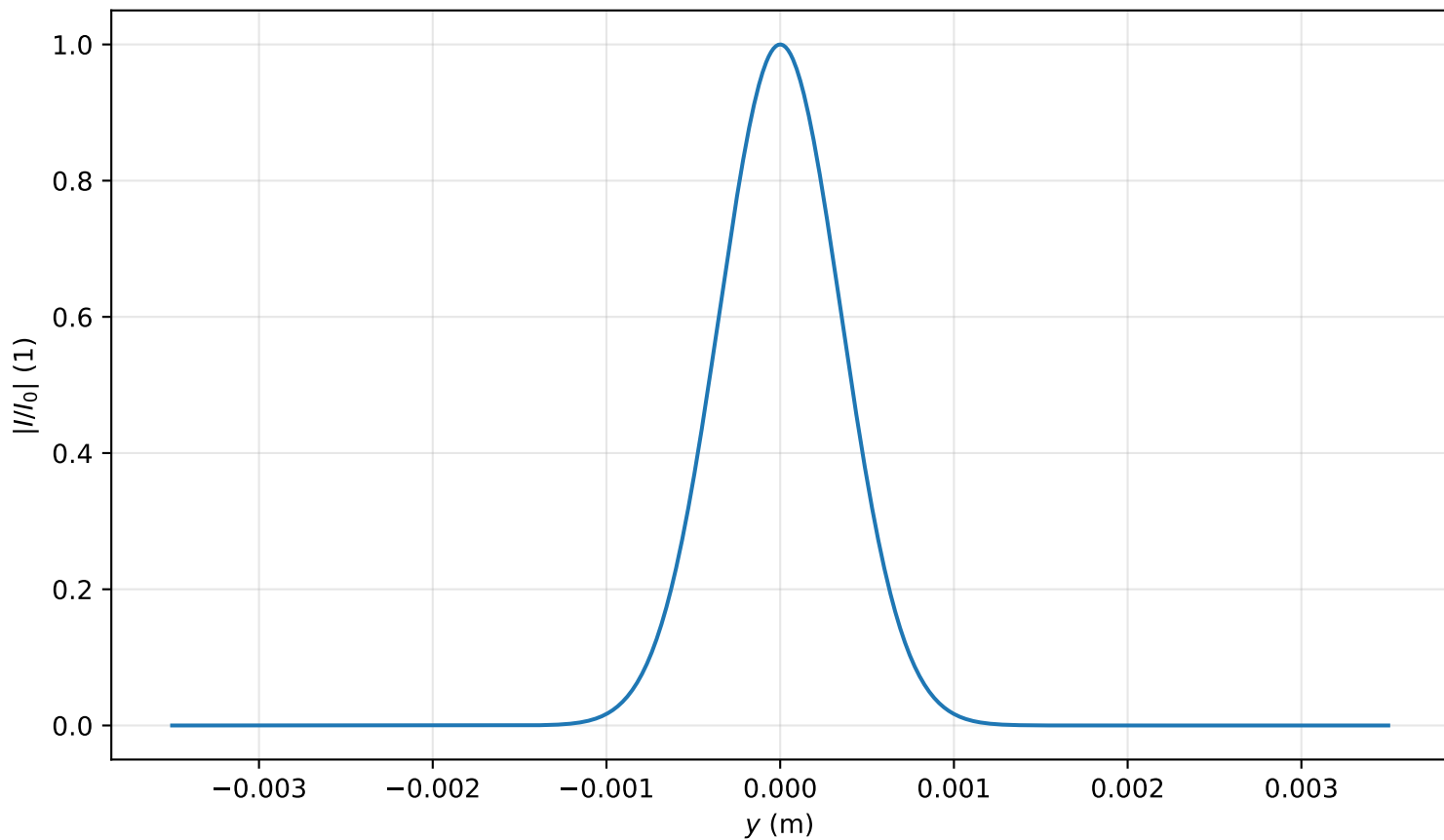
Intensity profile I(x=0, y, z=0.000)/I_0 , \text{Pin}=0.8\text{Pcr} , artificial time
